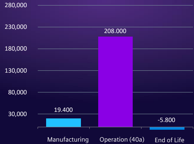
3AP1 DT 145 kV* enhanced design 2015 with mixed gas solution
